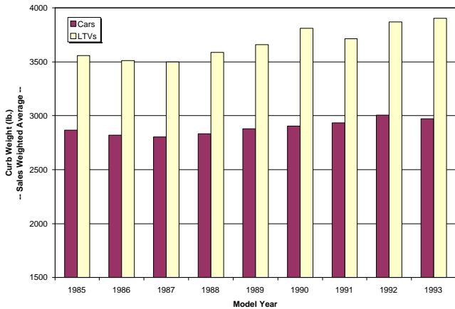
Figure 11. Sales-averaged Mass of LTVs and Passenger Cars from 1985-93 (Kahane, 1997).
