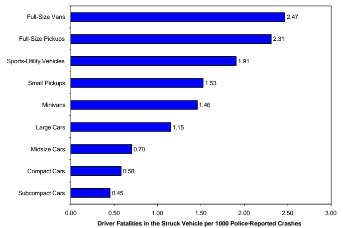
Figure 7. Vehicle Aggressivity by Vehicle Category (FARS/GES 1991-94).
