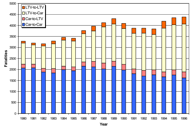
Figure 3. Distribution of Side Impact Fatalities (FARS 1980-96).
