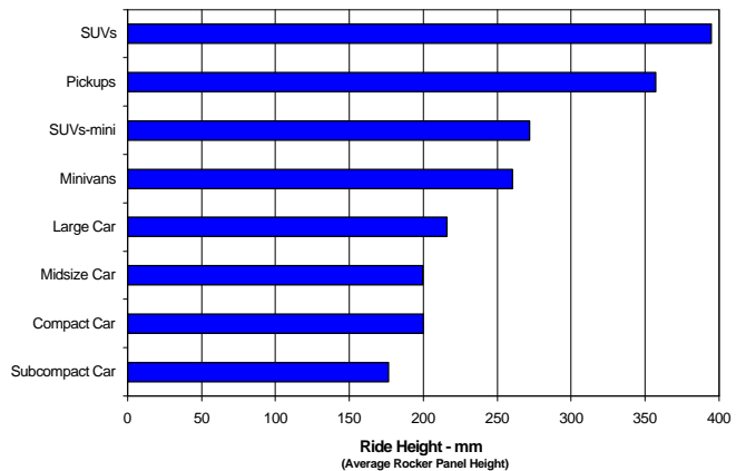
Figure 16. Geometric Compatibility: Average Ride Height vs. Vehicle Category as determined from AAMA Vehicle Specification Sheets (1990-94).
