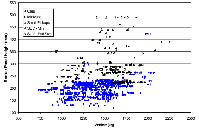
Figure 15. Relationship between Vehicle Mass and Ride Height as estimated by Rocker Panel Height. Reference: AAMA Vehicle Specification Sheets (1990-94).
