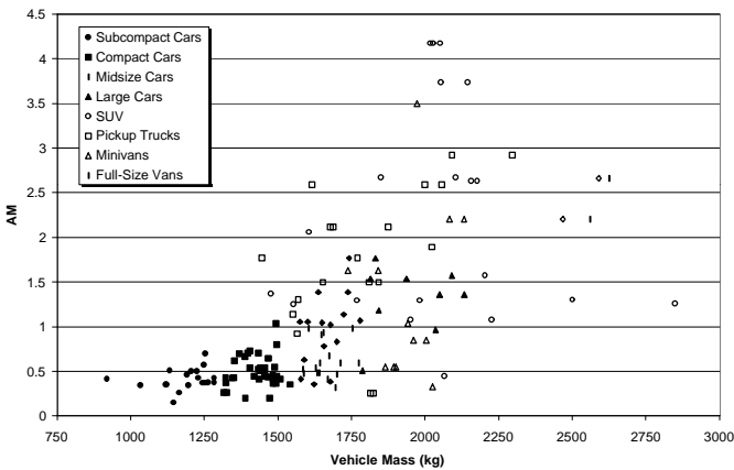
Figure 10. Aggressivity as a function of Vehicle Mass.
